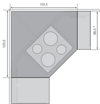
Dimensions worktop - Model 6211
