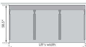
Dimensions worktop - Model 6210
