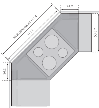
Dimensions worktop - Model 6212
