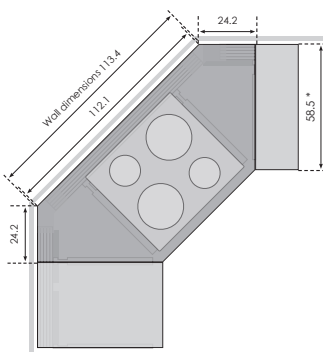
Dimensions worktop - Model 6202
