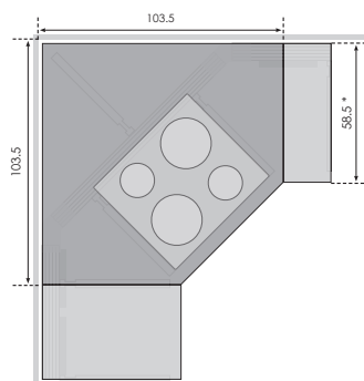
Dimensions worktop - Model 6201
